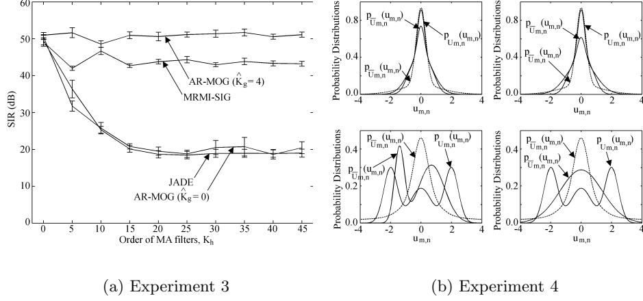
Fig. 2. (a) Separation performance as a function of K_h (the length of each h_m ) for Experiment 3. (b) Initial (dashed line) and final p_{\bar{U}_{m,n}}(u_{m,n}) distributions and p_{U_{m,n}}(u_{m,n}) for Experiment 4. Upper-left: Case 1. Upper-right: Case 2. Lower-left: Case 3. Lower-right: Case 4.
