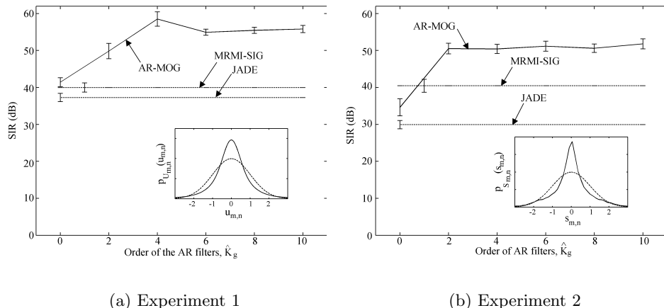
Fig. 1. Separation performance as a function of \hat{K}_g . (a) Experiment 1. The inset shows p_{u_{m,n}}(u_{m,n}) and a Gaussian distribution (dashed line) having the same mean and variance. (b) Experiment 2. The inset shows p_{s_{m,n}}(s_{m,n}) and a Gaussian distribution (dashed line) having the same mean and variance.
